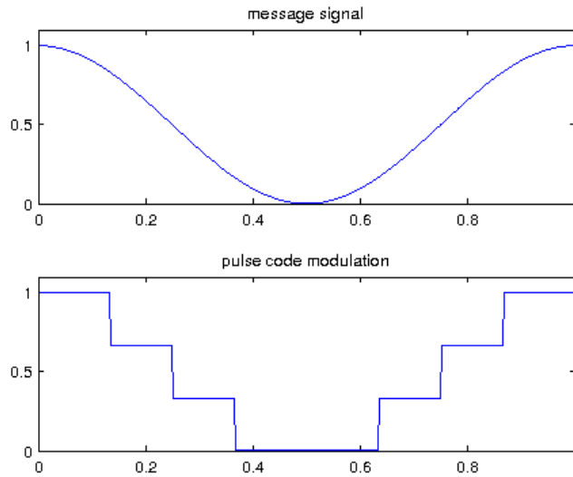
Figure 1: pulse code modulation with 2 bits
