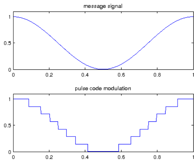
Figure 2: pulse code modulation with 3 bits
